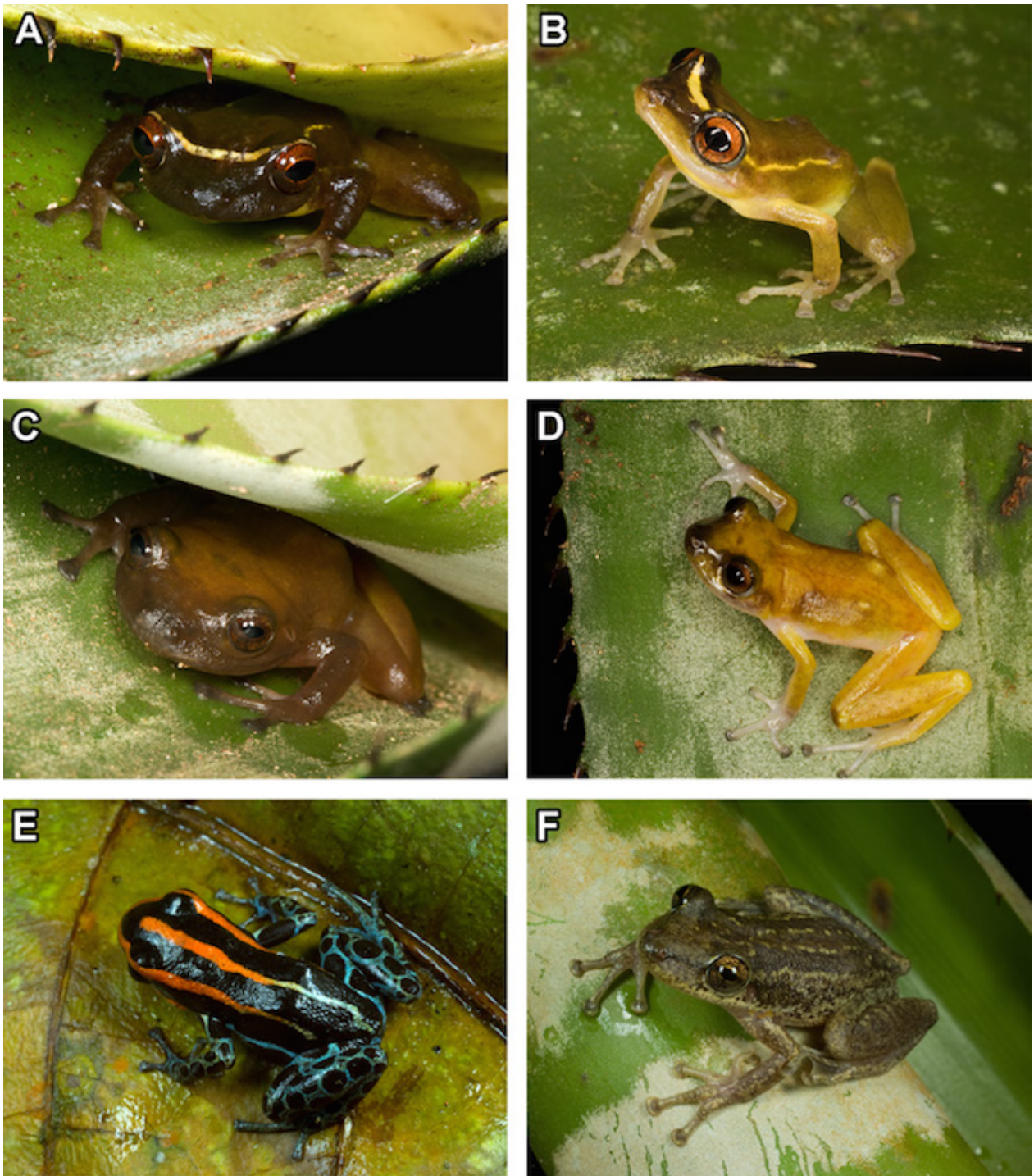
Fig. 3. A collection of anurans collected from Aechmea zebrina bromeliads. (A) Pristimantis aureolineatus hiding in leaf axil, and (B) on a leaf of A. zebrina . (C) Pristimantis waoranii emerging from leaf axil, and (D) on a leaf of A. zebrina . (E) Ranitomeya ventrimaculata and (F) Scinax ruber collected from A. zebrina bromeliads.
